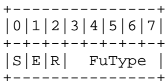
The Structure of FU Header
