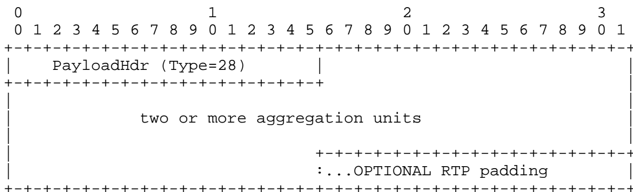
The Structure of an Aggregation Packet
