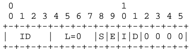
Short Frame Marking RTP Extension for [VVC]
